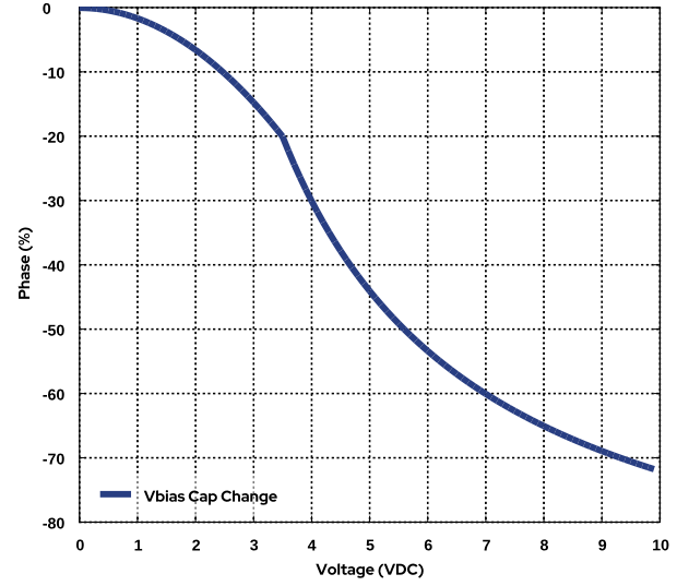
Capacitance Change vs. DC Voltage Bias
