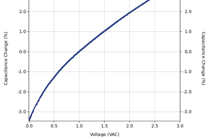
Capacitance Change versus AC Voltage
