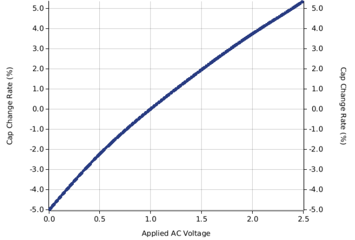
Capacitance Change vs. AC Voltage
