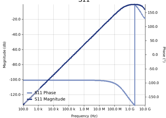
S11
