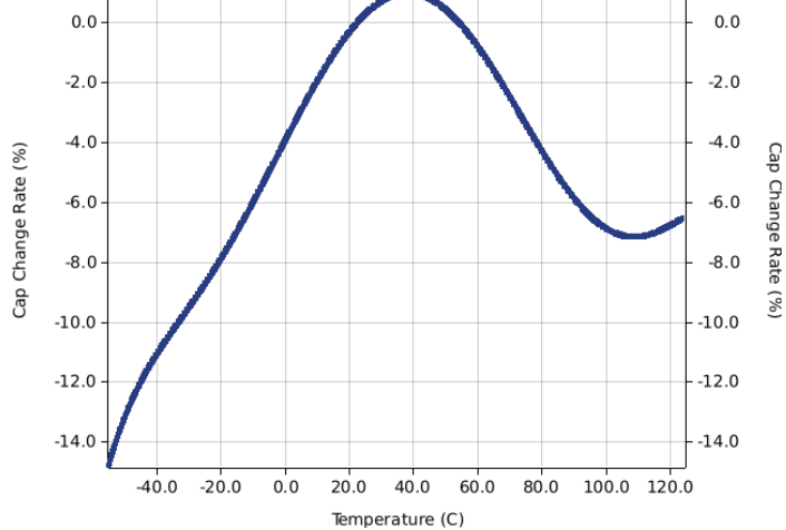
Capacitance Change vs. Temperature
