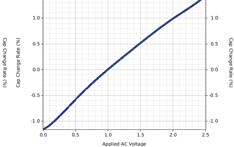
Capacitance Change vs. AC Voltage
