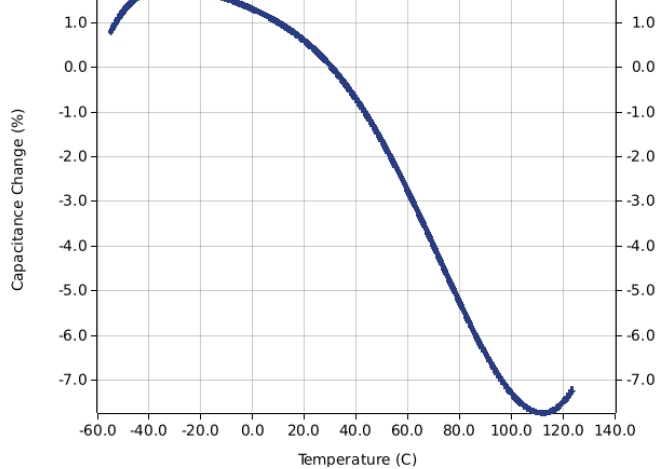
Capacitance Change versus Temperature
