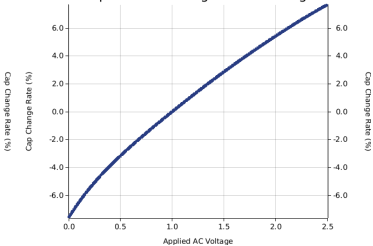
Capacitance Change vs. AC Voltage
