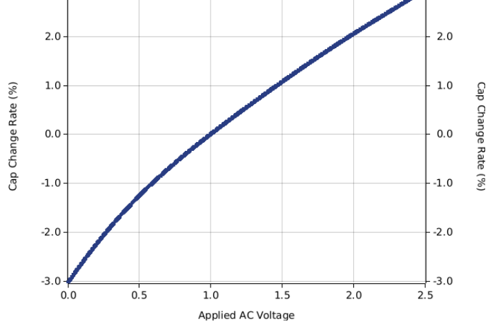
Capacitance Change vs. AC Voltage
