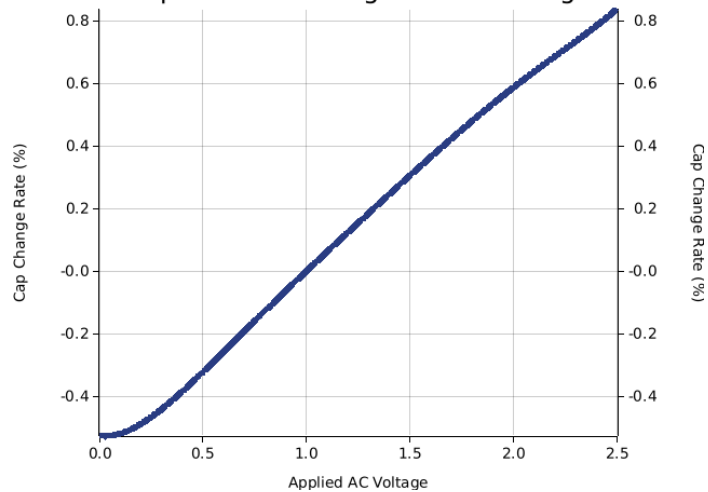
Capacitance Change vs. AC Voltage
